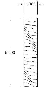
5-1/2" flat casing
