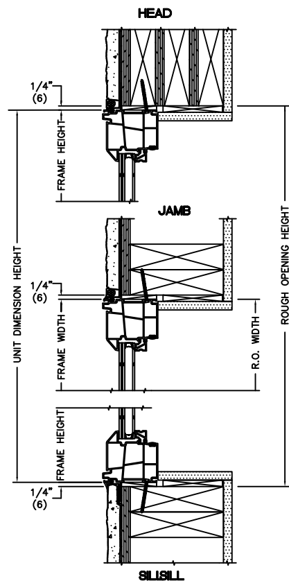
Stucco finish over 1/2" sheathing 2 x 6 frame wall with drywall return.
