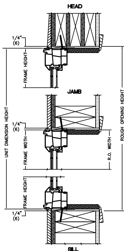
Wood lap siding over 1/2" sheathing 2 x 6 wood frame with extension jamb and 1/2" drywall.
