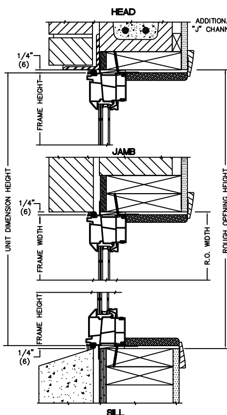
Brick veneer over 6" masonry wall with wide extension jamb and 1/2" drywall.
