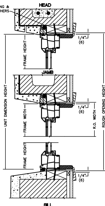
Stucco exterior finish over 8" masonry block wall with extension jamb and 1/2" drywall.
