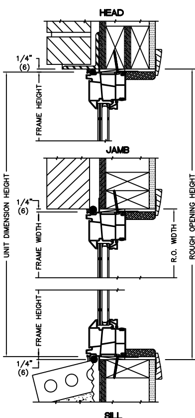
Brick veneer over 1/2" sheathing, 2 x 4 wood frame and 1/2" drywall.
