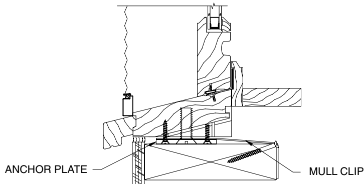
SILL STEEL REINFORCED MULLION (INSTALLATION BY OTHERS)
