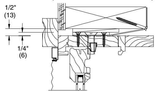
HEAD STEEL REINFORCED MULLION (INSTALLATION BY OTHERS)
