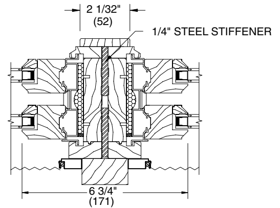
SECTION DETAIL 1/4" STEEL REINFORCED MULLION (FACTORY OR FIELD APPLIED)
