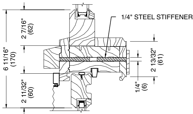
SECTION DETAIL 1/4" STEEL REINFORCED MULLION (FACTORY OR FIELD APPLIED)
