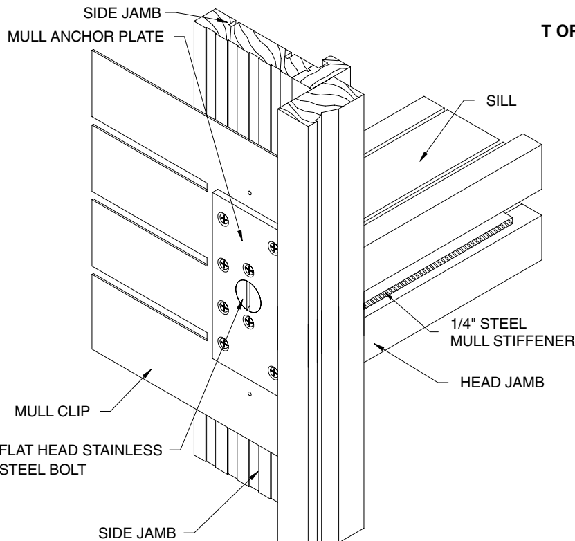
SILL STEEL REINFORCED MULLION (INSTALLATION BY OTHERS)
